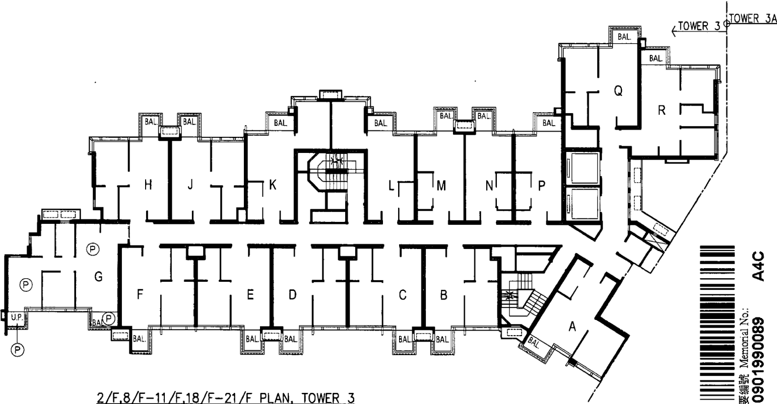
2/F, 8/F-11/F, 18/F-21/F PLAN, TOWER 3
