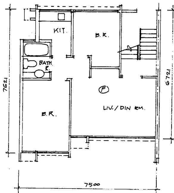
PLAN HOUSE 1
