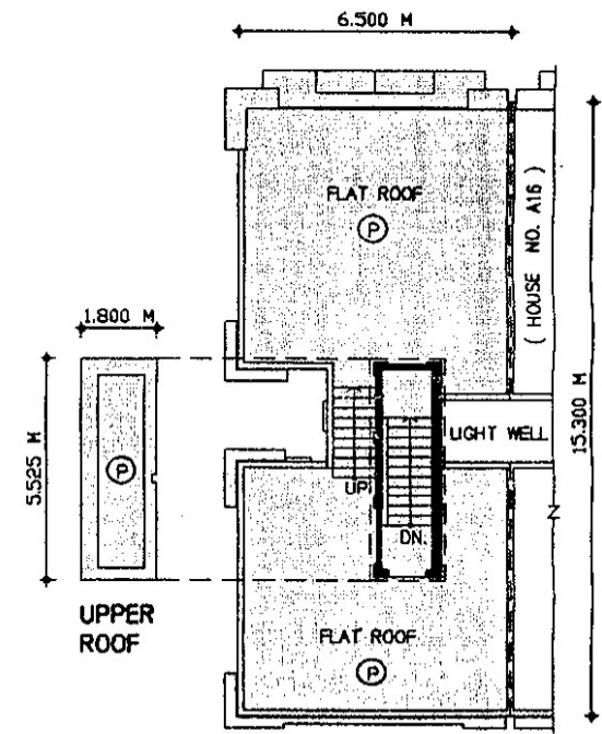
ROOF PLAN
