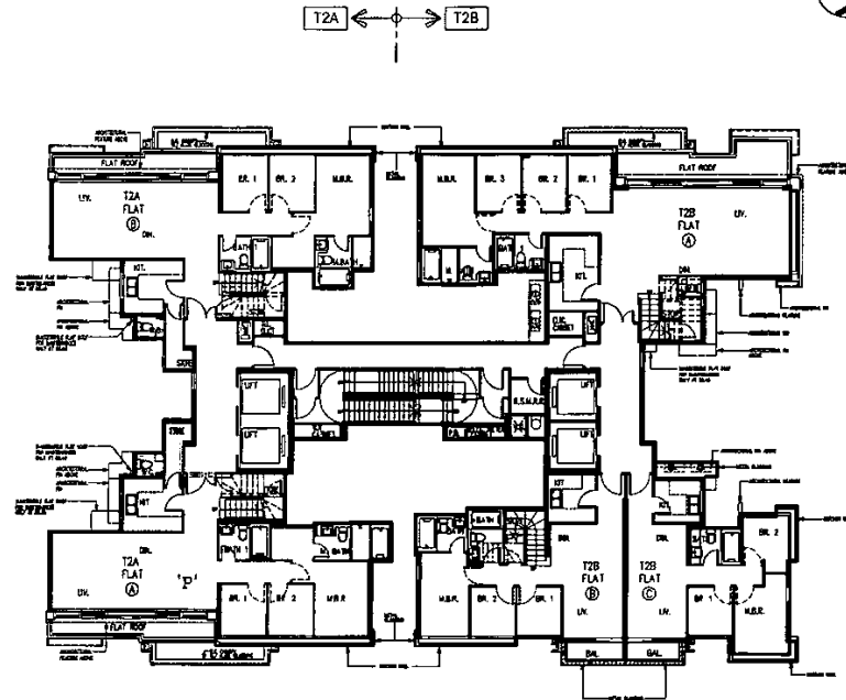
18TH FLOOR PLAN
