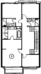
FIRST FLOOR
