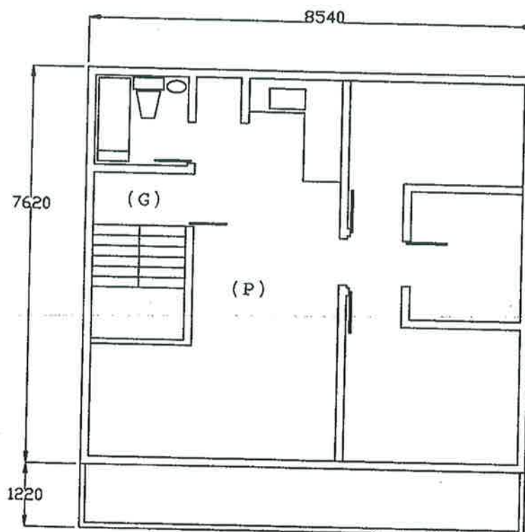
1/F PLAN
