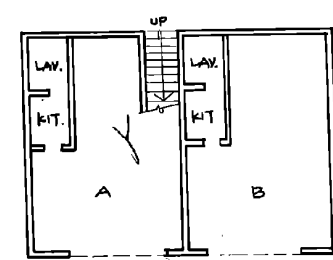
GROUND FLOOR BLOCK 'A' PLAN
