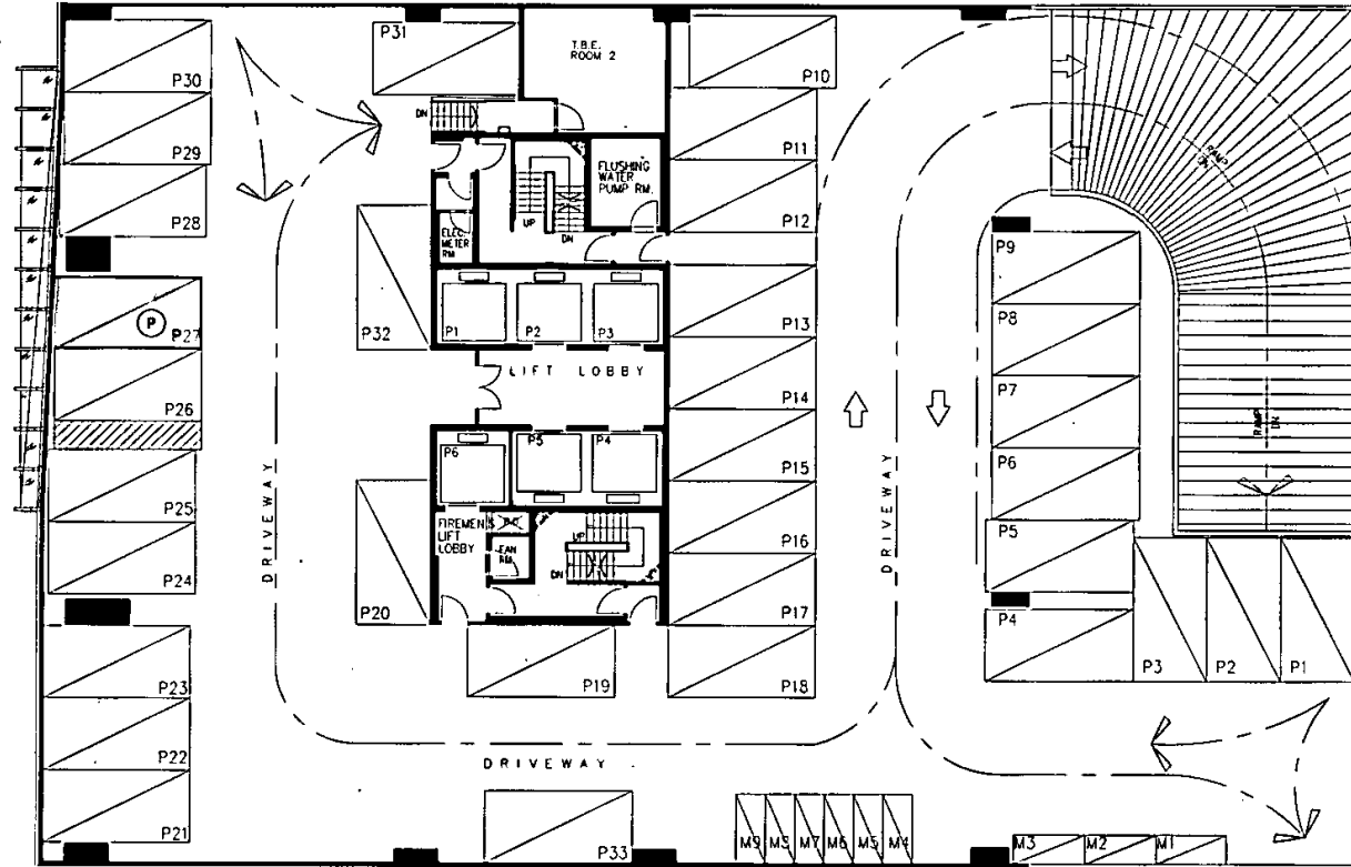
3/F PLAN
