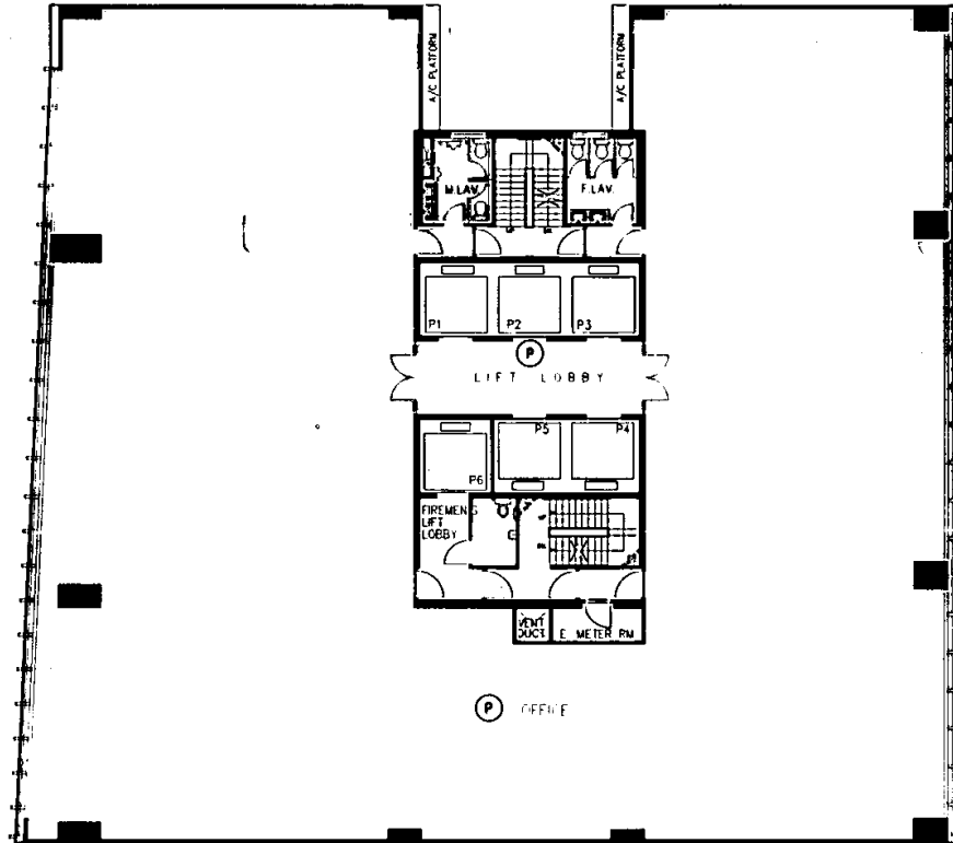
11/F PLAN
