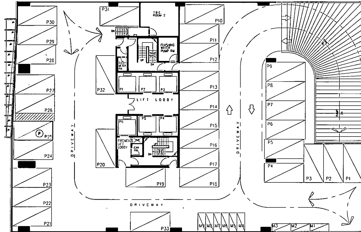
3/F PLAN
