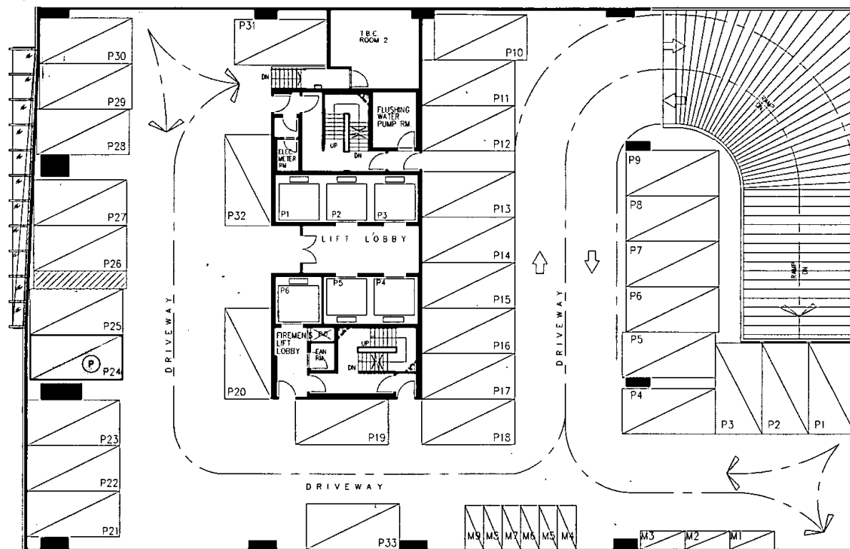
3/F PLAN
