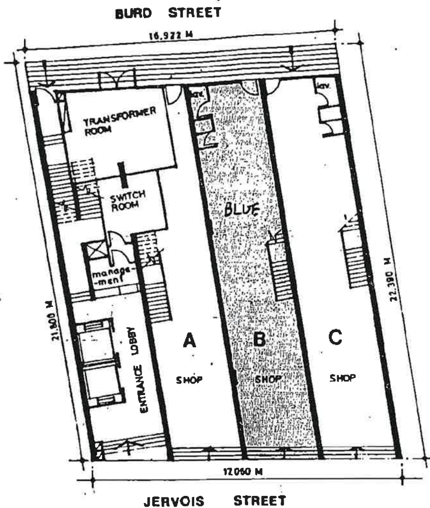
GROUND FLOOR PLAN SHOP NO. B SCALE 1:200
