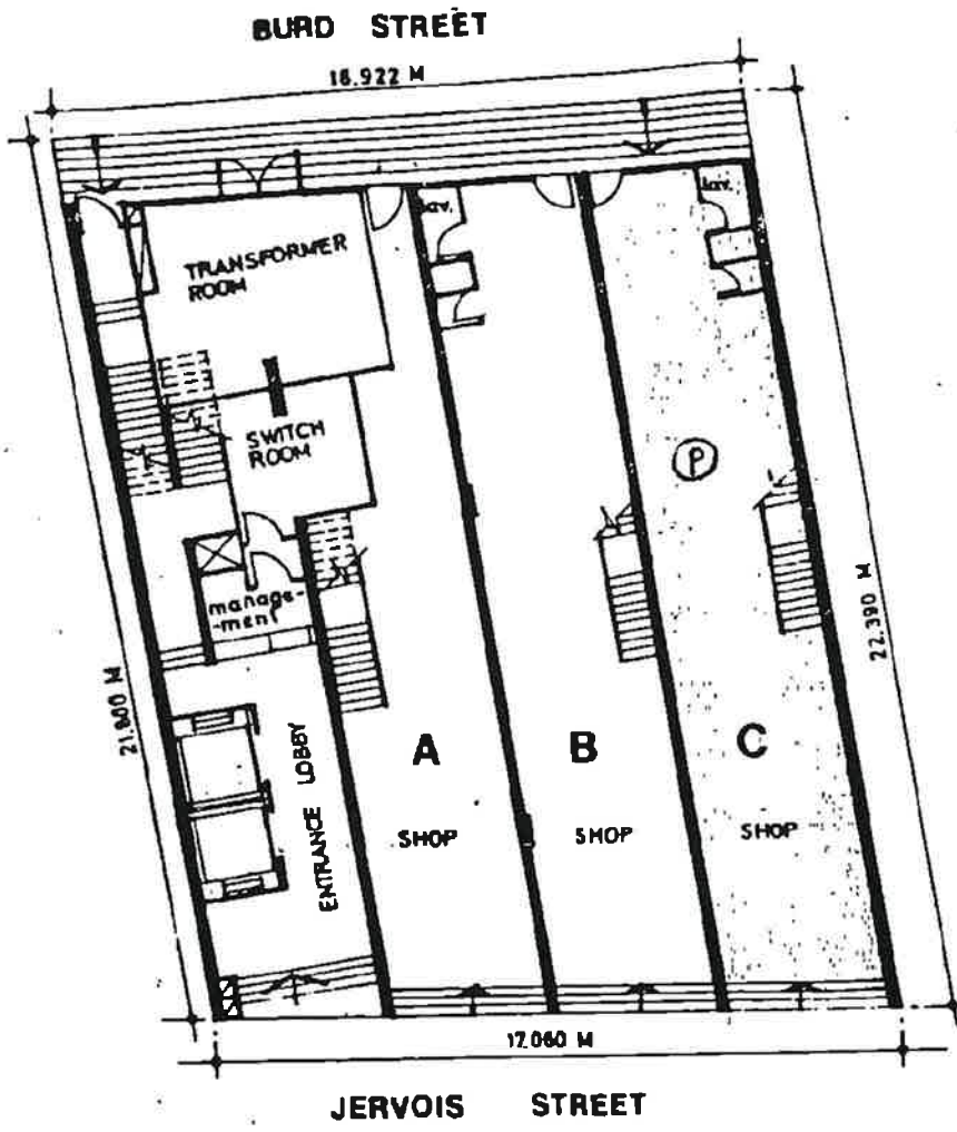
GROUND FLOOR PLAN SHOP NO. C SCALE 1:200
