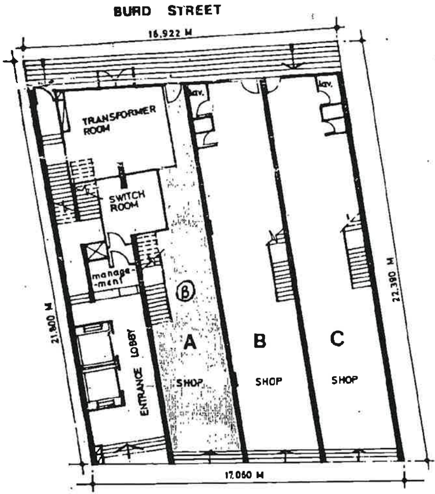
GROUND FLOOR PLAN SHOP NO. A SCALE 1:200
