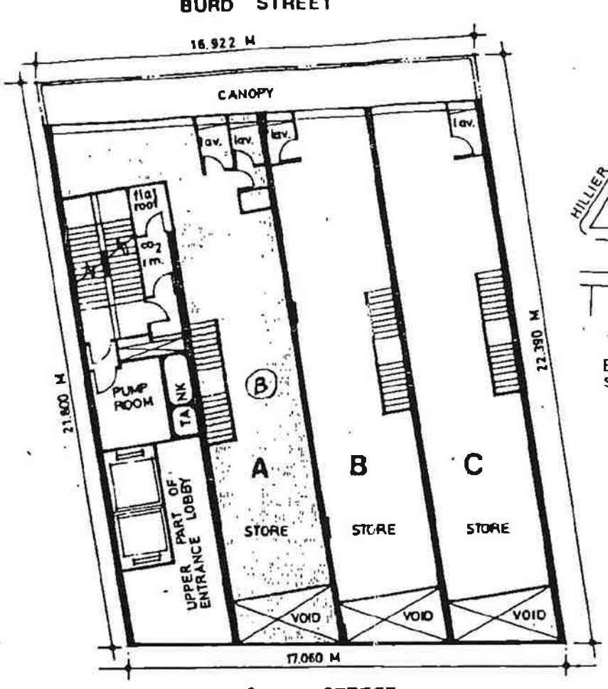
MEZZ FLOOR PLAN SHOP NO. A SCALE 1:200
