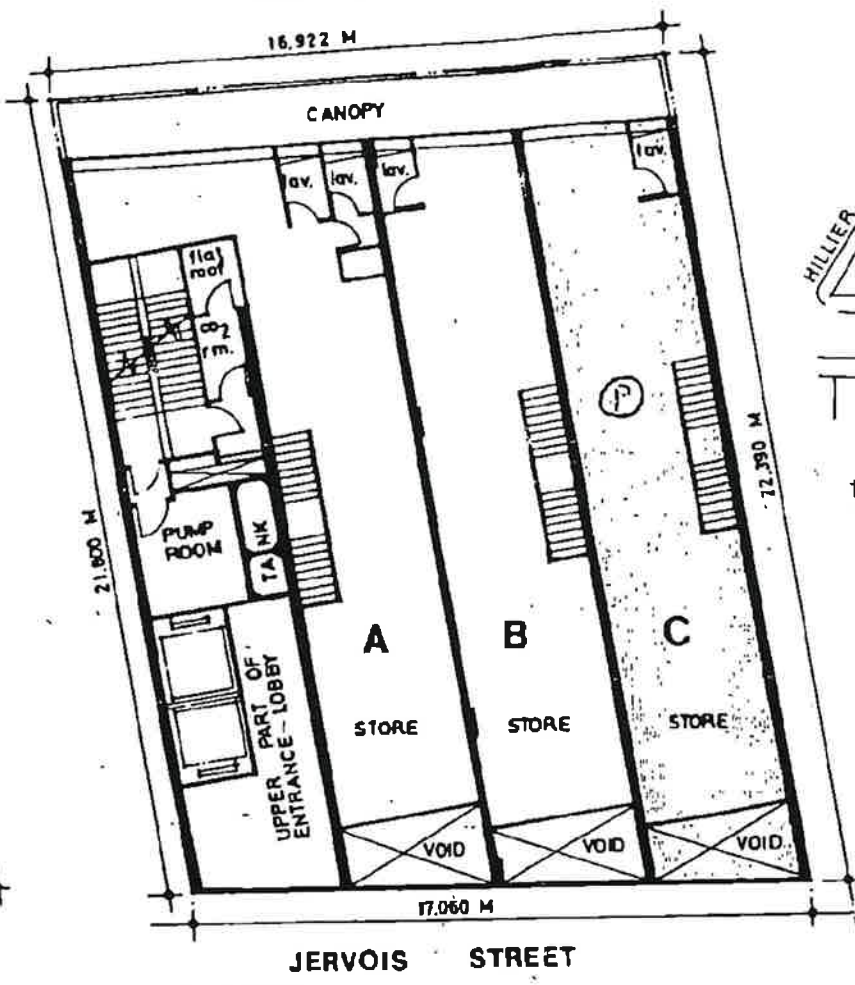
MEZZ FLOOR PLAN SHOP NO. C SCALE 1:200
