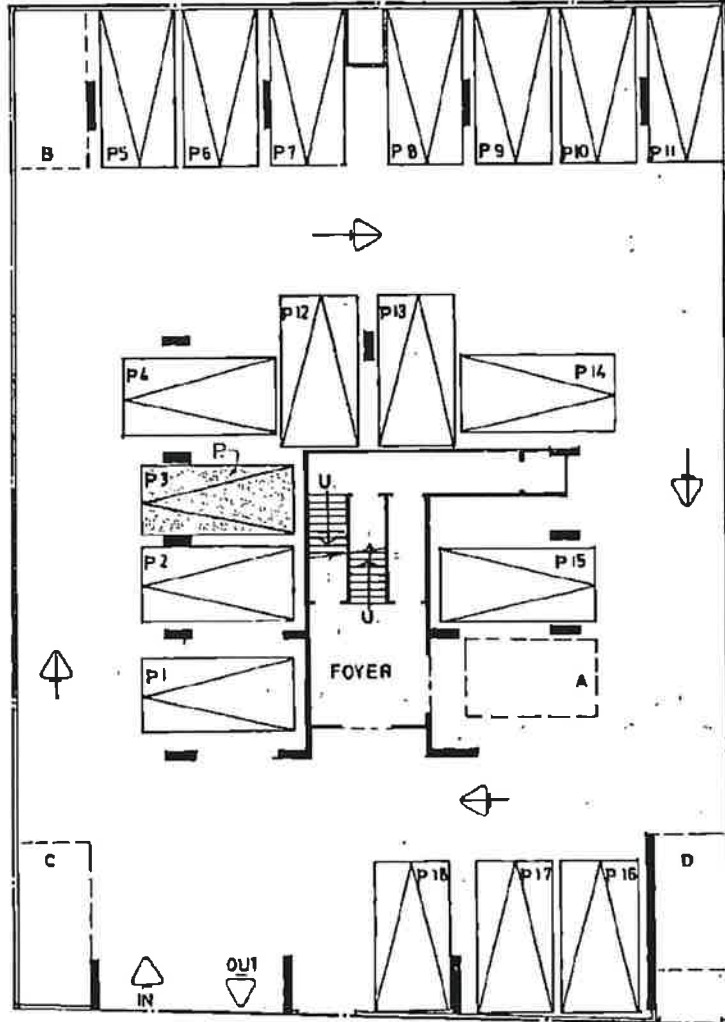
TAT CHEE AVENUE GROUND FLOOR PLAN
