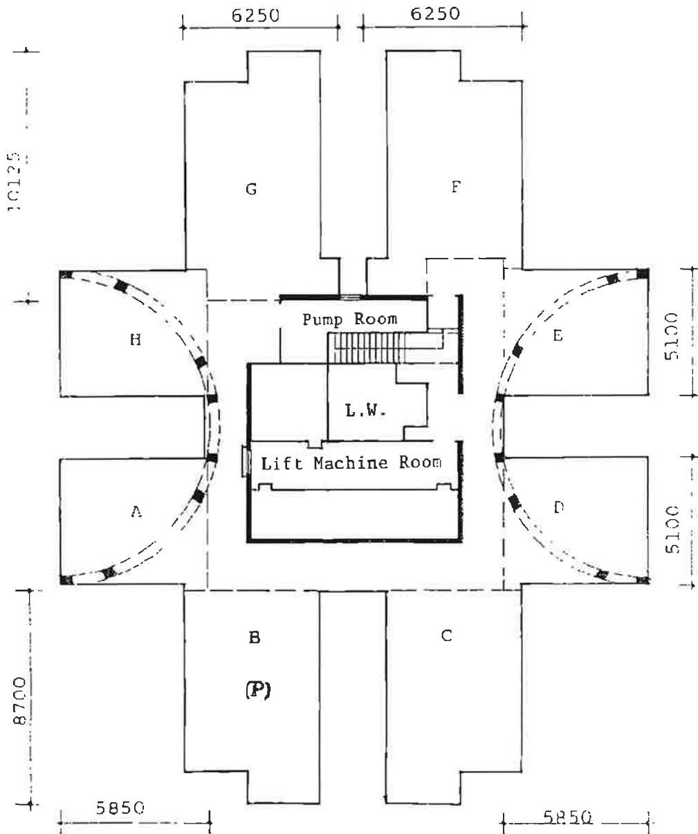
Roof Plan
