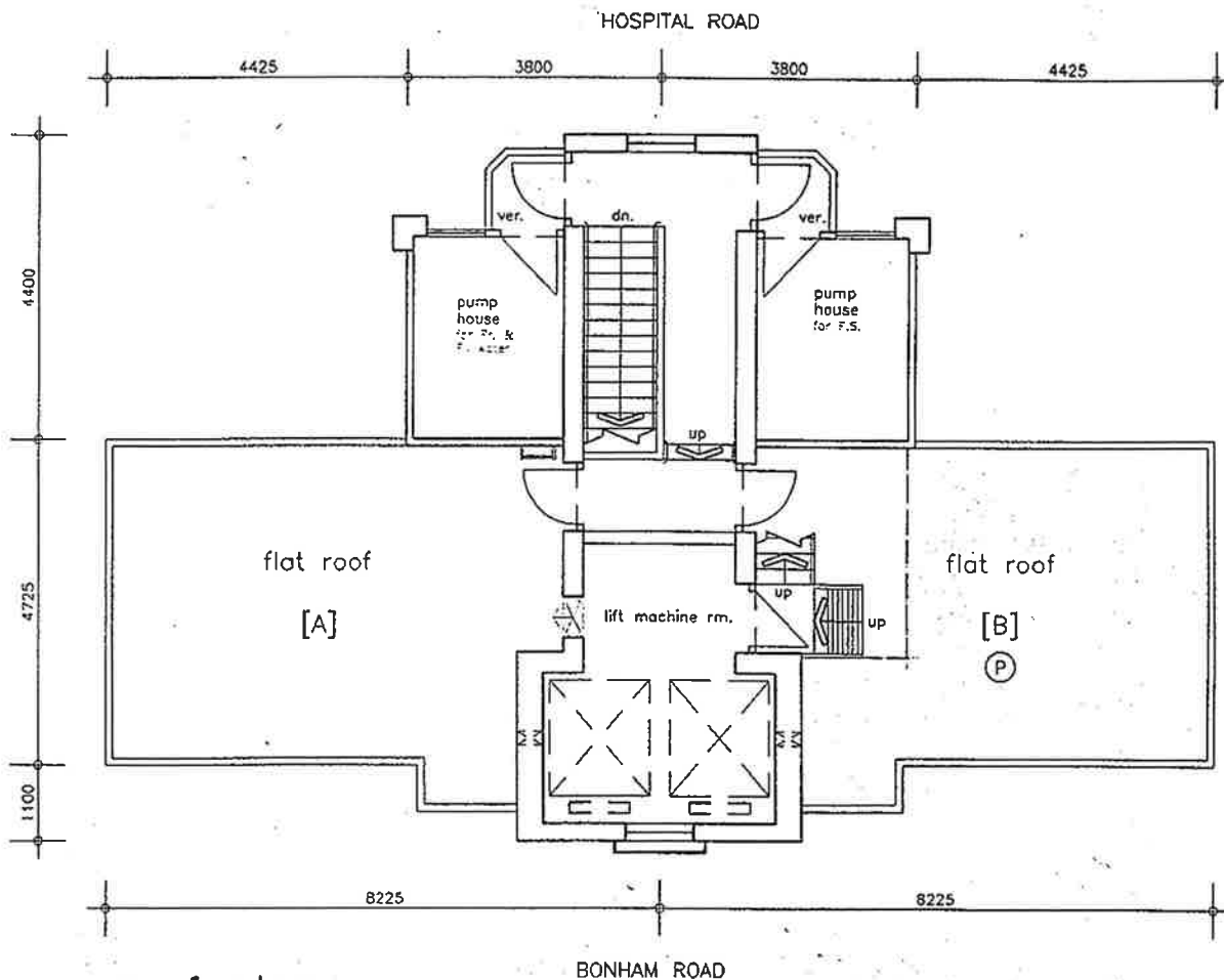
roof plan
