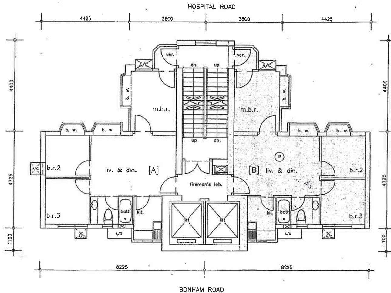
32nd floor plan
